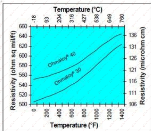
Resistivity as a Function of Temperature
